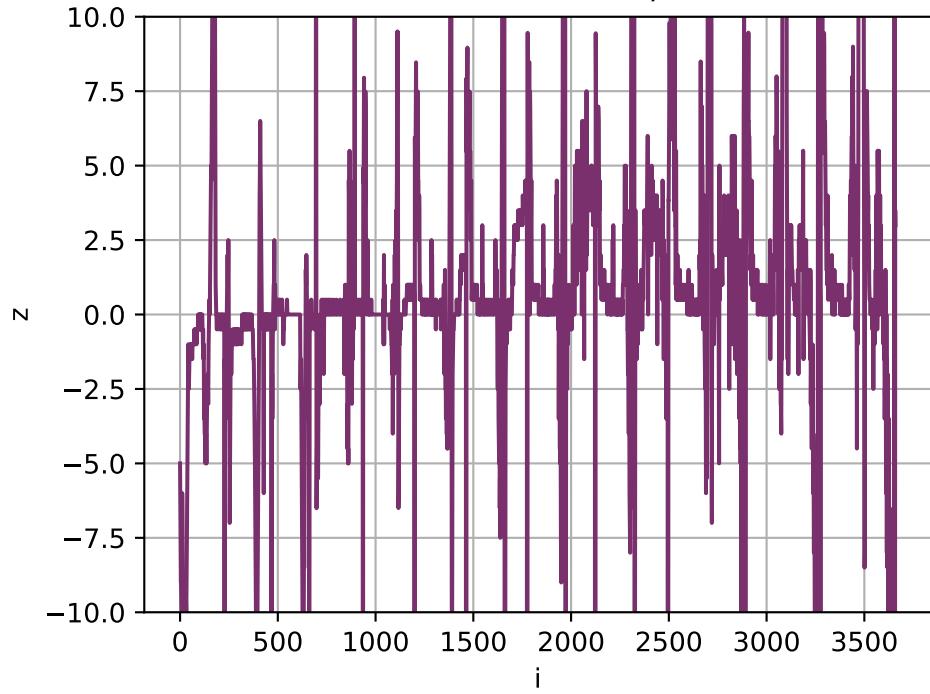
Derivative z = d\delta/dx
